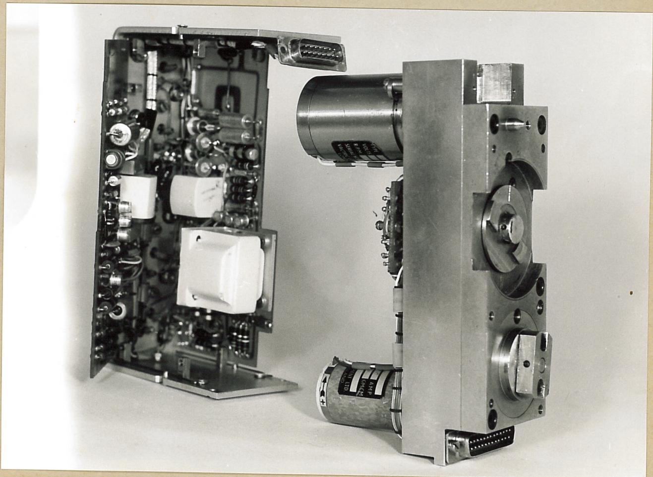
HF - SSB SERVO-MECHANISM.
