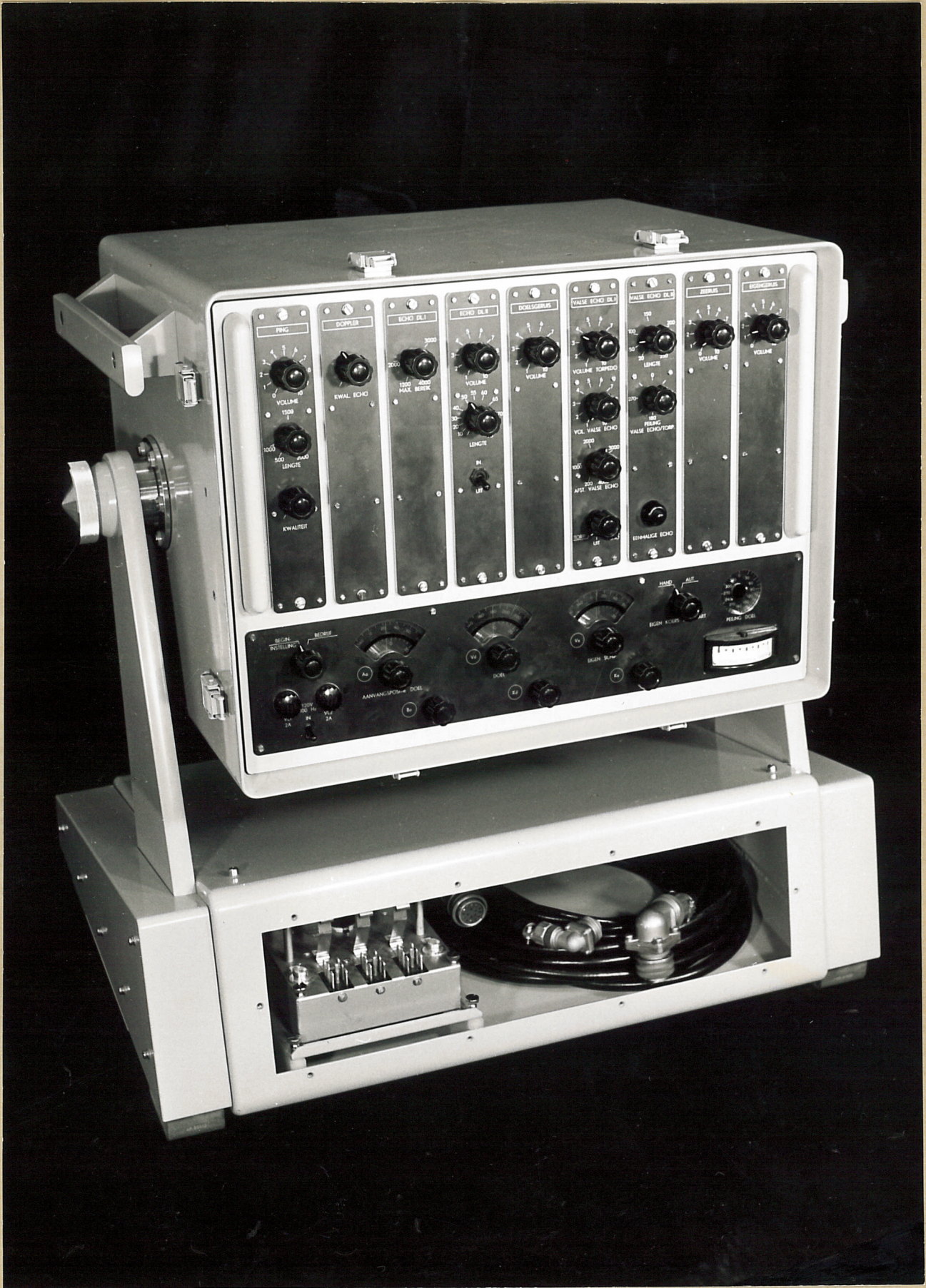
SSI TRANSISTORIZED, PORTABLE SONAR SIMULATOR
